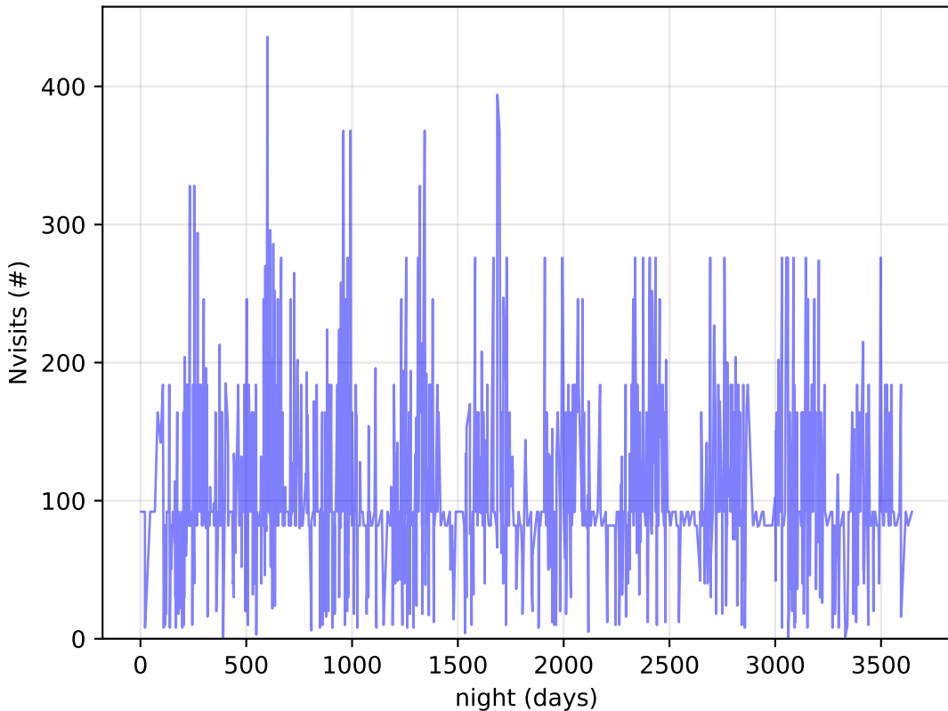
roll_uniform_eh_acc0.2_mjdp0_v3.4_10yrs DDF: Nvisits
