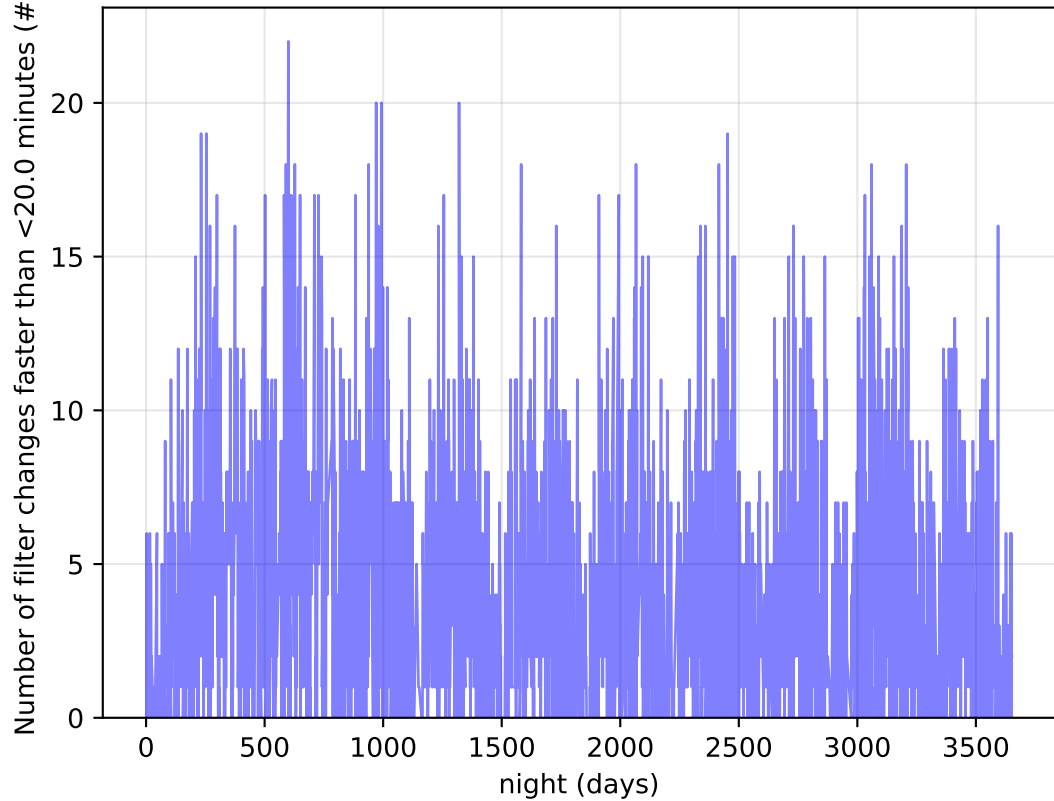
roll_uniform_eh_acc0.2_mjdp0_v3.4_10yrs Per Night: Number of filter changes faster than <20.0 minutes
