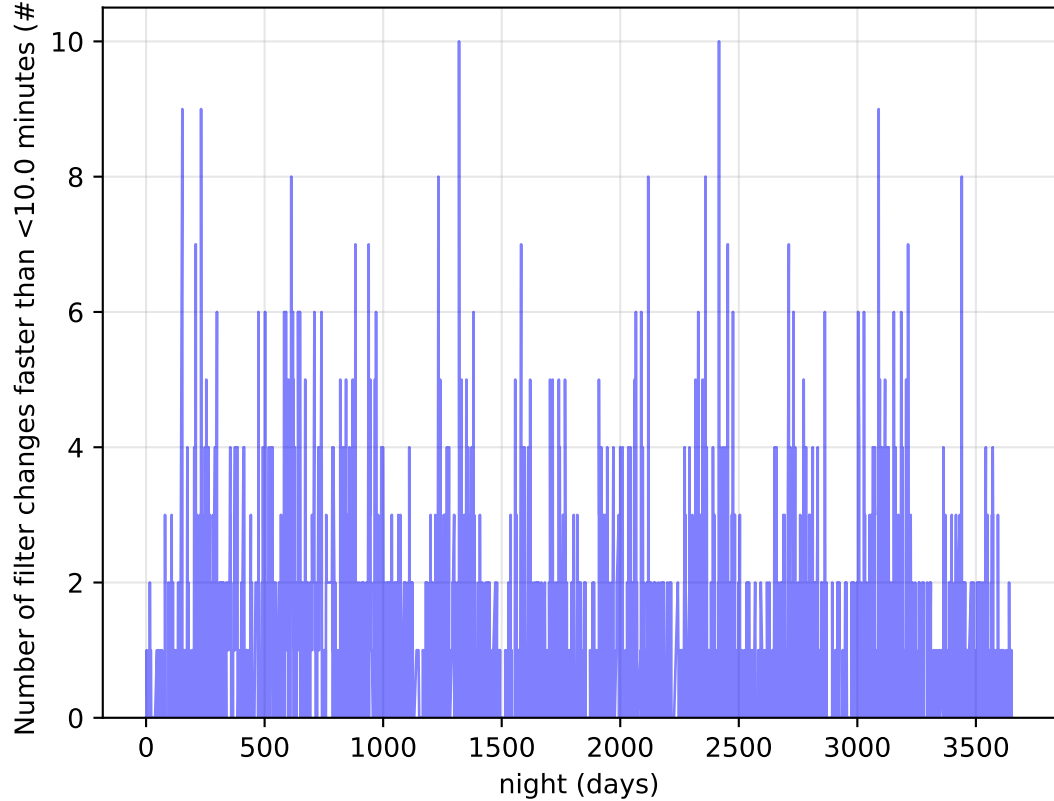
roll_uniform_eh_acc0.2_mjdp0_v3.4_10yrs Per Night: Number of filter changes faster than <10.0 minutes
