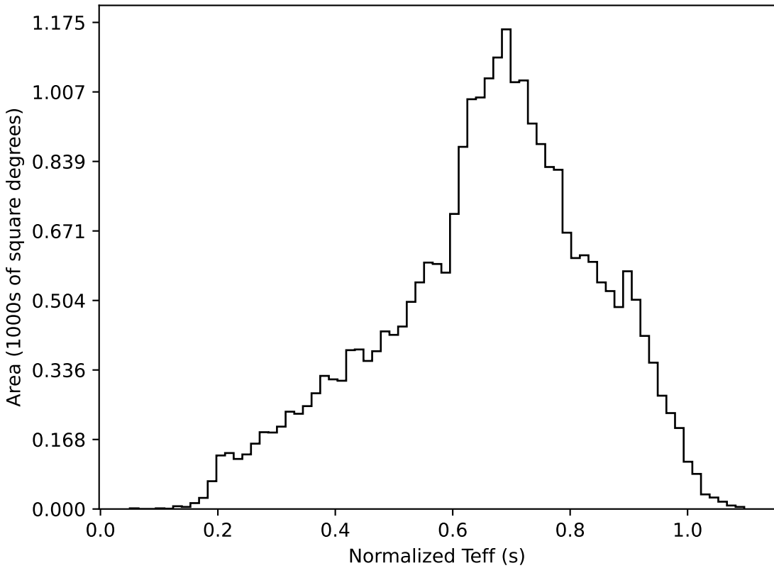
roll_uniform_eh_acc0.2_mjdp0_v3.4_10yrs All sky all bands: Normalized Teff
