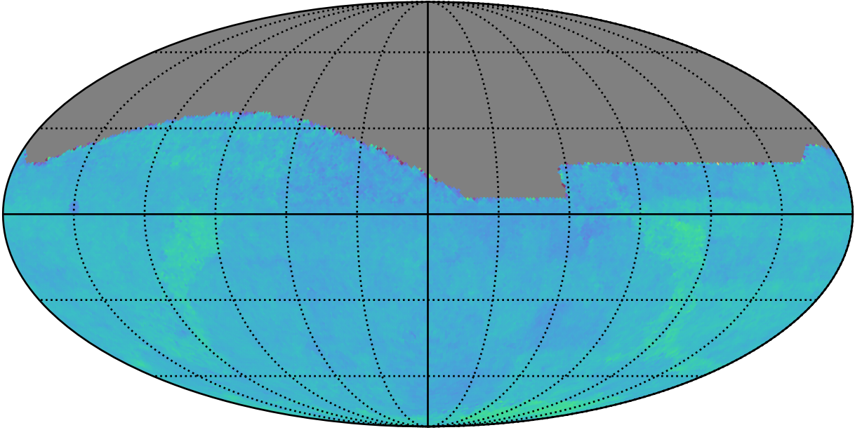
roll_uniform_eh_acc0.2_mjdp0_v3.4_10yrs All sky: Normalized Proper Motion Uncert @ 24.0
