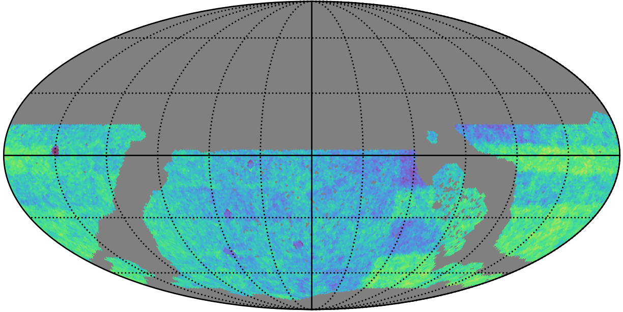
roll_uniform_eh_acc0.2_mjdp0_v3.4_10yrs WFD: Normalized Proper Motion Uncert @ 20.5
