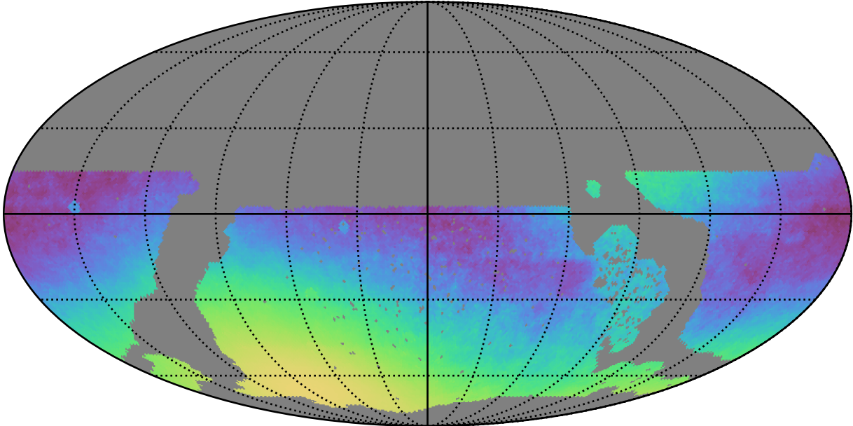
roll_uniform_eh_acc0.2_mjdp0_v3.4_10yrs WFD: Normalized Parallax Uncert @ 24.0
