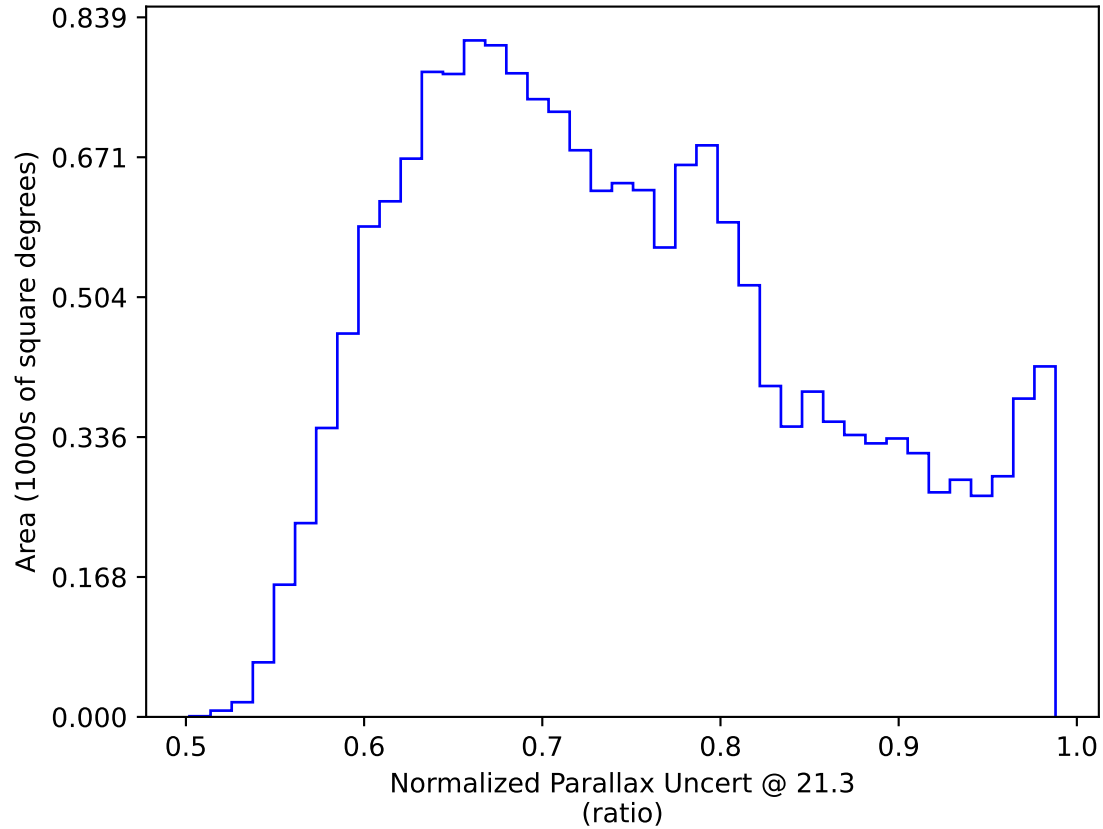
roll_uniform_eh_acc0.2_mjdp0_v3.4_10yrs WFD y band only: Normalized Parallax Uncert @ 21.3
