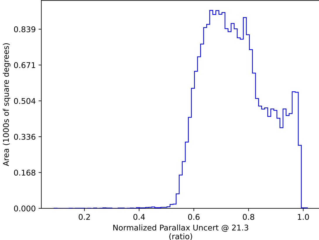
roll_uniform_eh_acc0.2_mjdp0_v3.4_10yrs All sky y band only: Normalized Parallax Uncert @ 21.3
