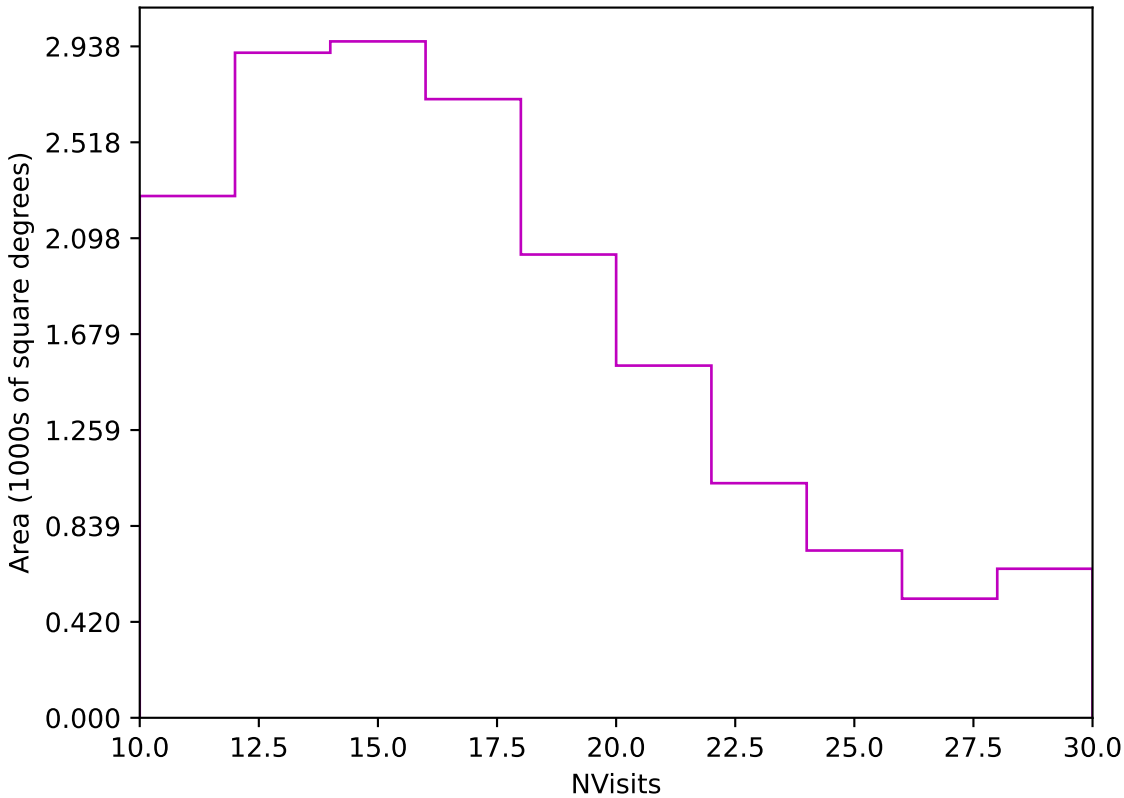
roll_uniform_eh_acc0.2_mjdp0_v3.4_10yrs Yr 3-4 z band: NVisits
