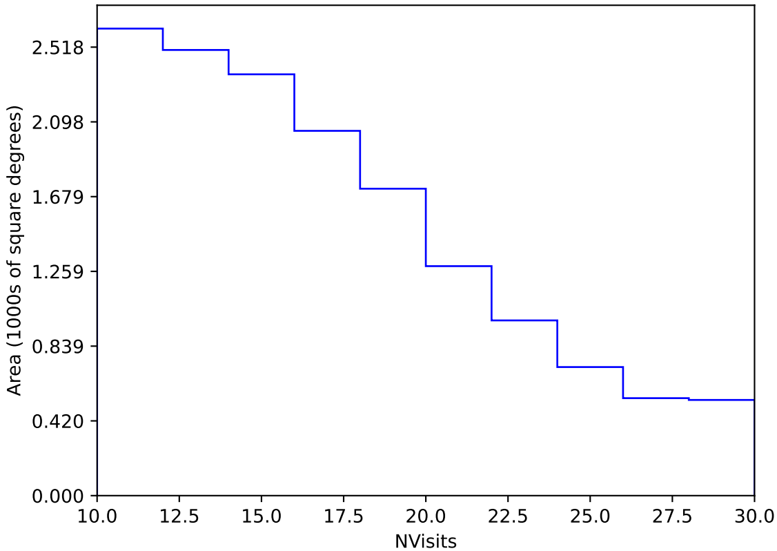
roll_uniform_eh_acc0.2_mjdp0_v3.4_10yrs Yr 3-4 y band: NVisits
