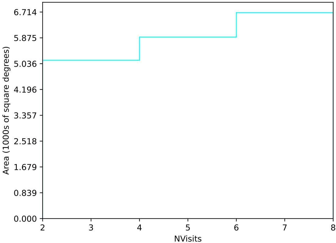
roll_uniform_eh_acc0.2_mjdp0_v3.4_10yrs Yr 3-4 u band: NVisits
