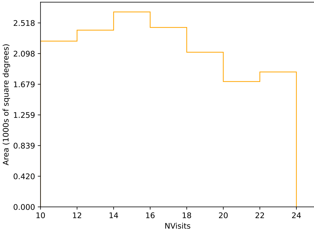
roll_uniform_eh_acc0.2_mjdp0_v3.4_10yrs Yr 3-4 r band: NVisits
