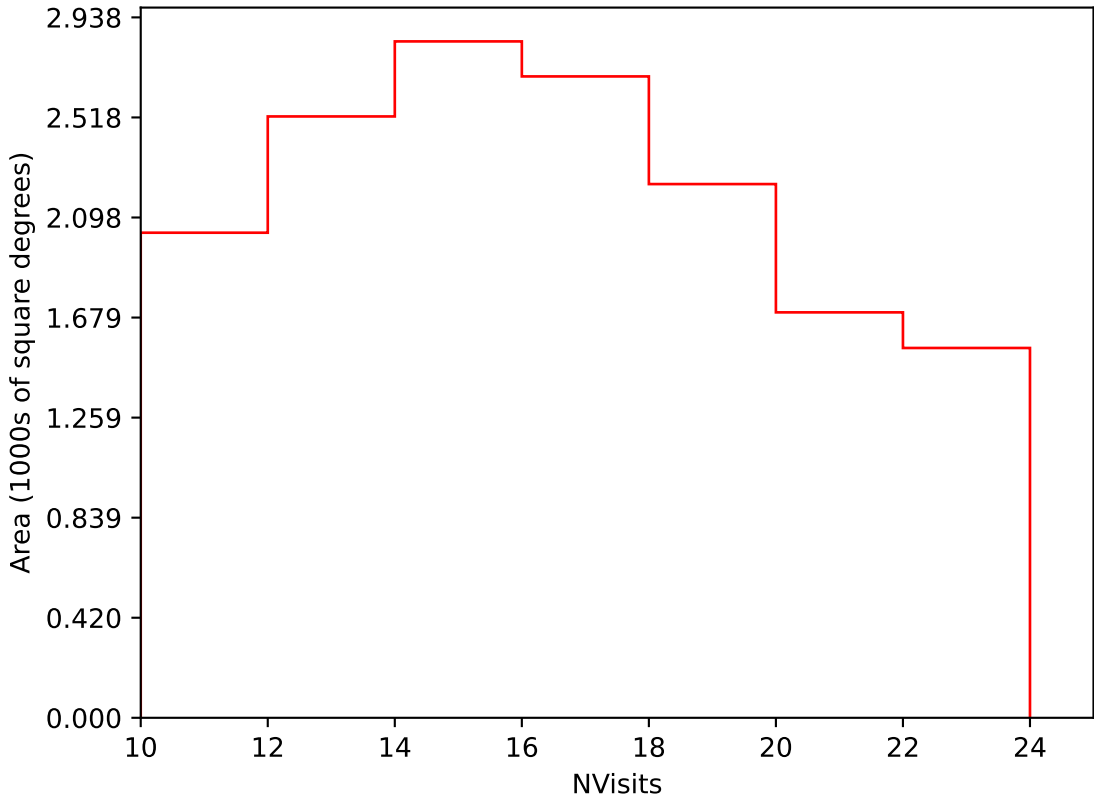
roll_uniform_eh_acc0.2_mjdp0_v3.4_10yrs Yr 3-4 i band: NVisits
