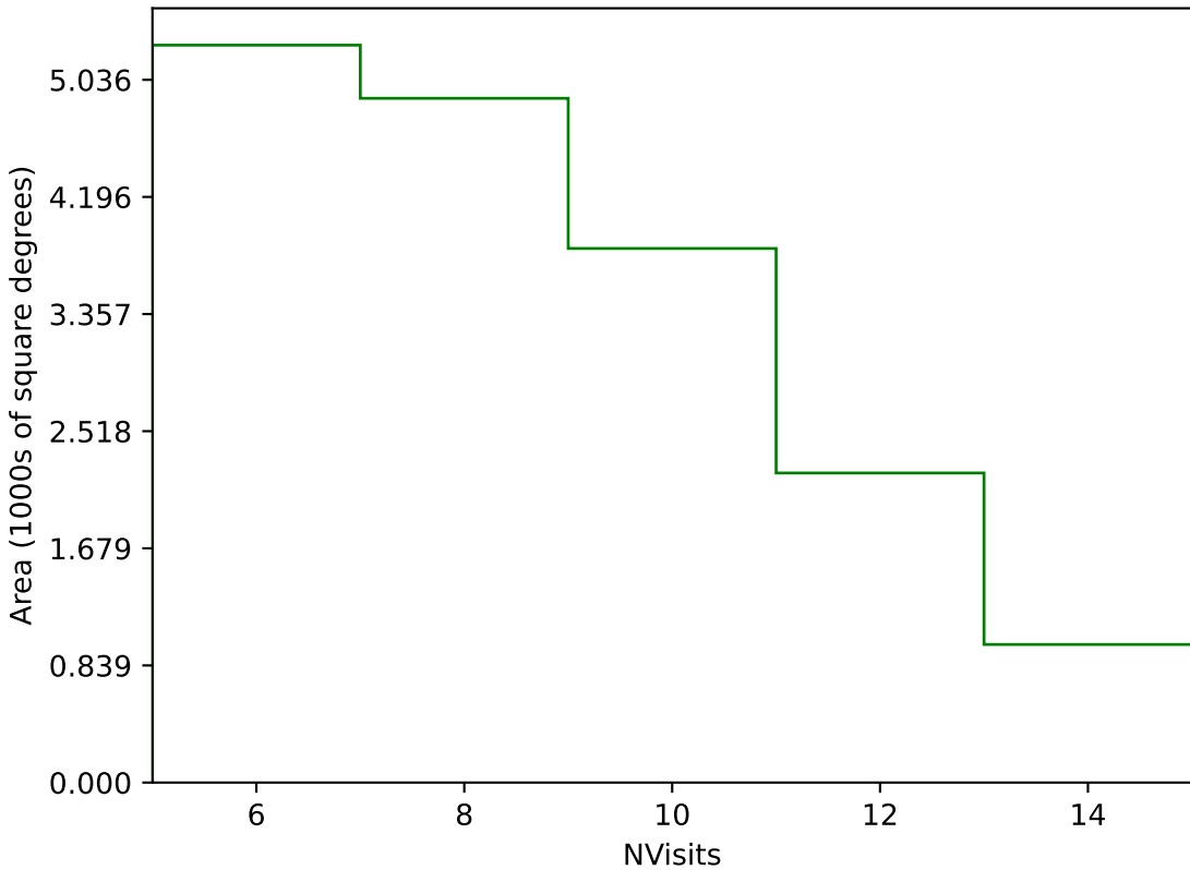
roll_uniform_eh_acc0.2_mjdp0_v3.4_10yrs Yr 3-4 g band: NVisits
