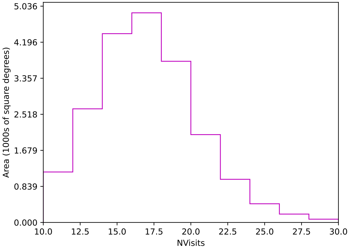
roll_uniform_eh_acc0.2_mjdp0_v3.4_10yrs Yr 1 z band: NVisits
