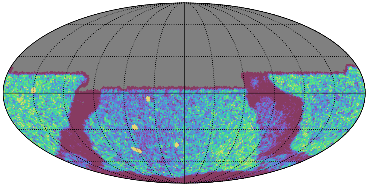
roll_uniform_eh_acc0.2_mjdp0_v3.4_10yrs Yr 1 y band: NVisits
