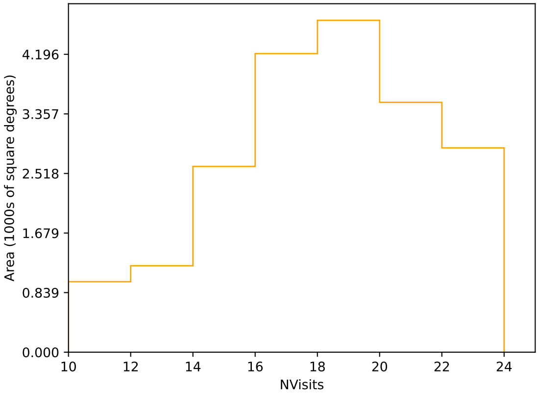
roll_uniform_eh_acc0.2_mjdp0_v3.4_10yrs Yr 1 r band: NVisits
