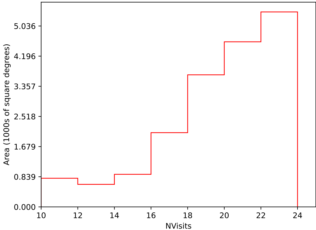
roll_uniform_eh_acc0.2_mjdp0_v3.4_10yrs Yr 1 i band: NVisits
