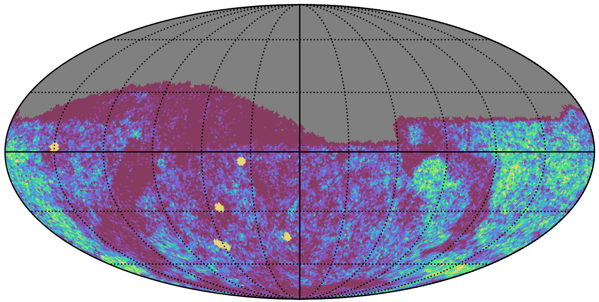
roll_uniform_eh_acc0.2_mjdp0_v3.4_10yrs Yr 1 g band: NVisits
