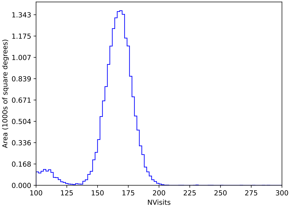
roll_uniform_eh_acc0.2_mjdp0_v3.4_10yrs WFD y band: NVisits
