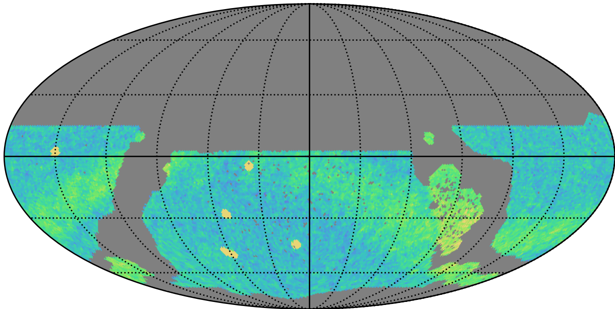
roll_uniform_eh_acc0.2_mjdp0_v3.4_10yrs WFD r band: NVisits
