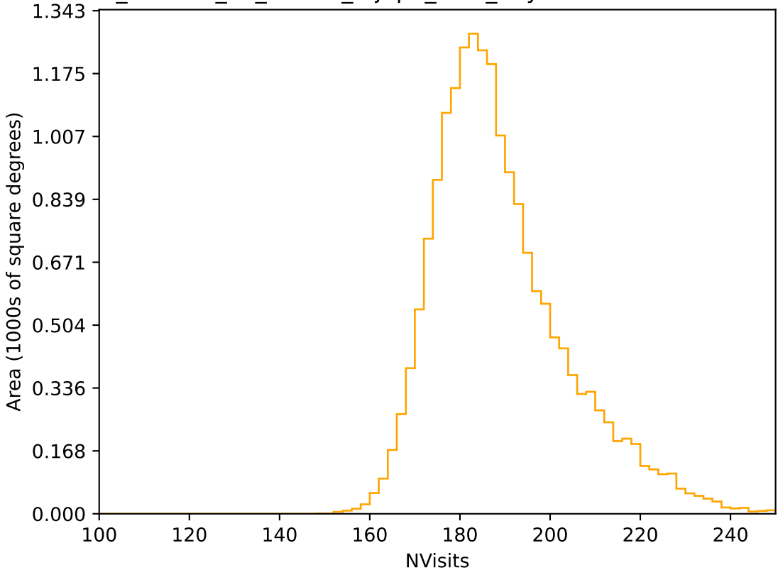
roll_uniform_eh_acc0.2_mjdp0_v3.4_10yrs WFD r band: NVisits
