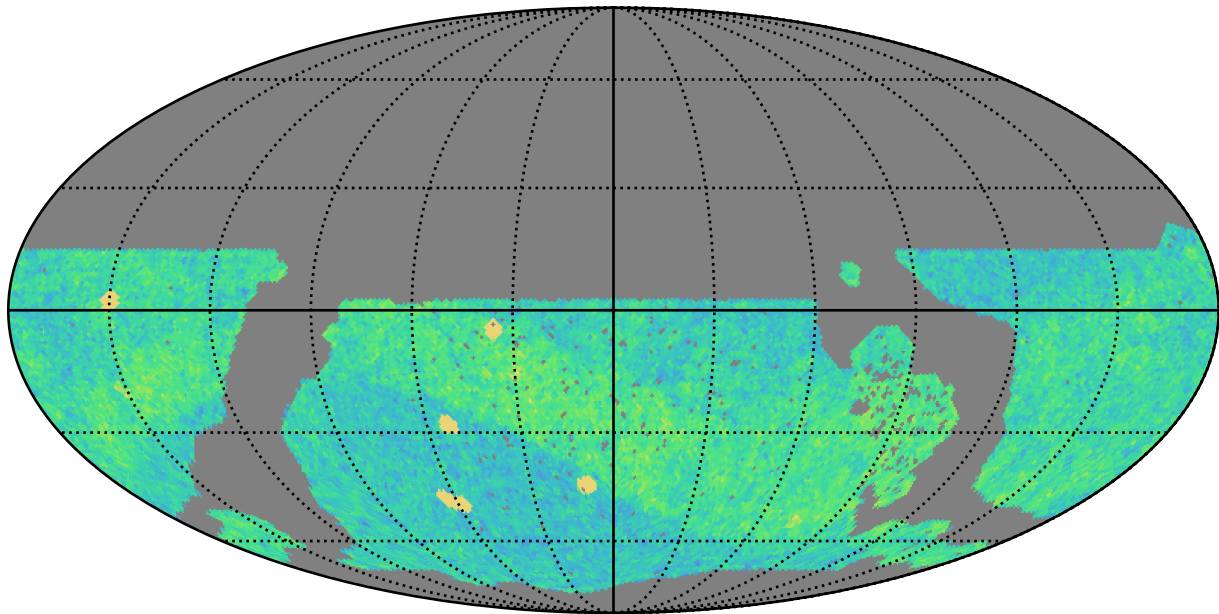
roll_uniform_eh_acc0.2_mjdp0_v3.4_10yrs WFD i band: NVisits
