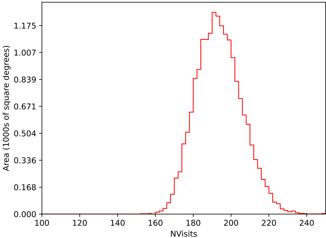
roll_uniform_eh_acc0.2_mjdp0_v3.4_10yrs WFD i band: NVisits
