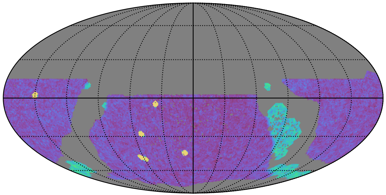
roll_uniform_eh_acc0.2_mjdp0_v3.4_10yrs WFD g band: NVisits
