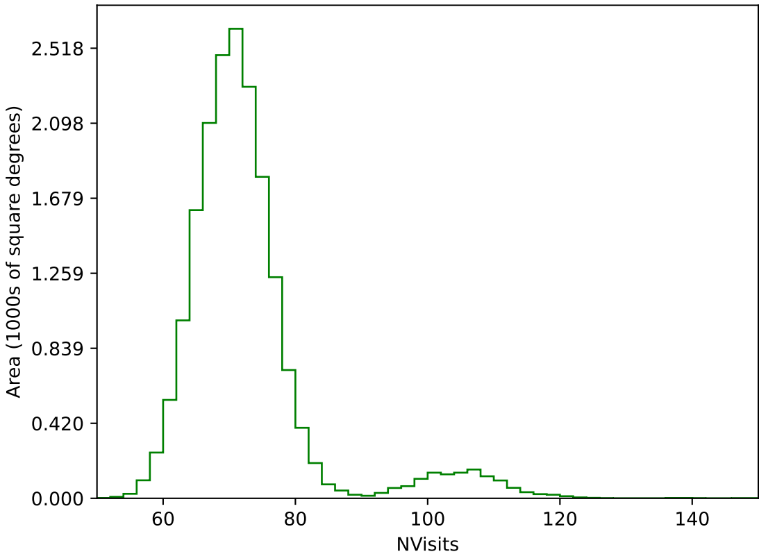
roll_uniform_eh_acc0.2_mjdp0_v3.4_10yrs WFD g band: NVisits
