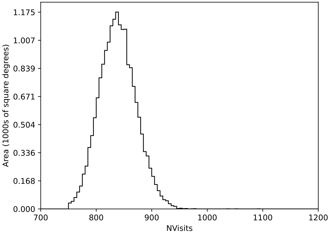
roll_uniform_eh_acc0.2_mjdp0_v3.4_10yrs WFD all bands: NVisits
