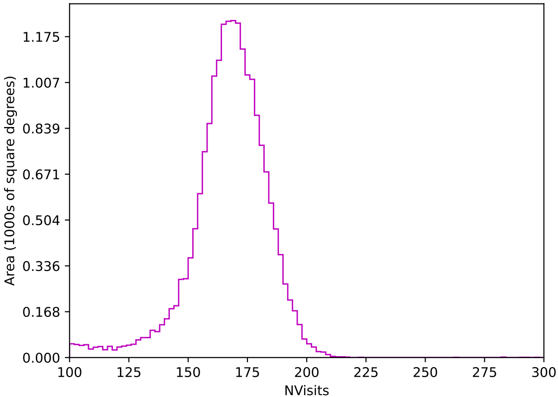
roll_uniform_eh_acc0.2_mjdp0_v3.4_10yrs All sky z band: NVisits
