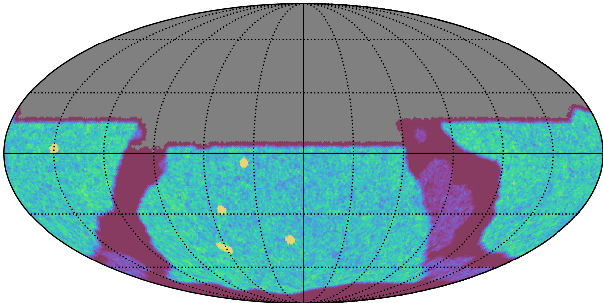
roll_uniform_eh_acc0.2_mjdp0_v3.4_10yrs All sky u band: NVisits
