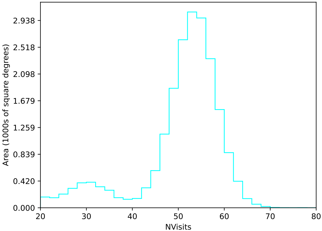
roll_uniform_eh_acc0.2_mjdp0_v3.4_10yrs All sky u band: NVisits
