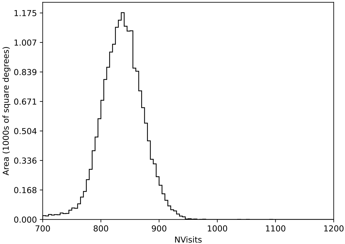
roll_uniform_eh_acc0.2_mjdp0_v3.4_10yrs All sky all bands: NVisits
