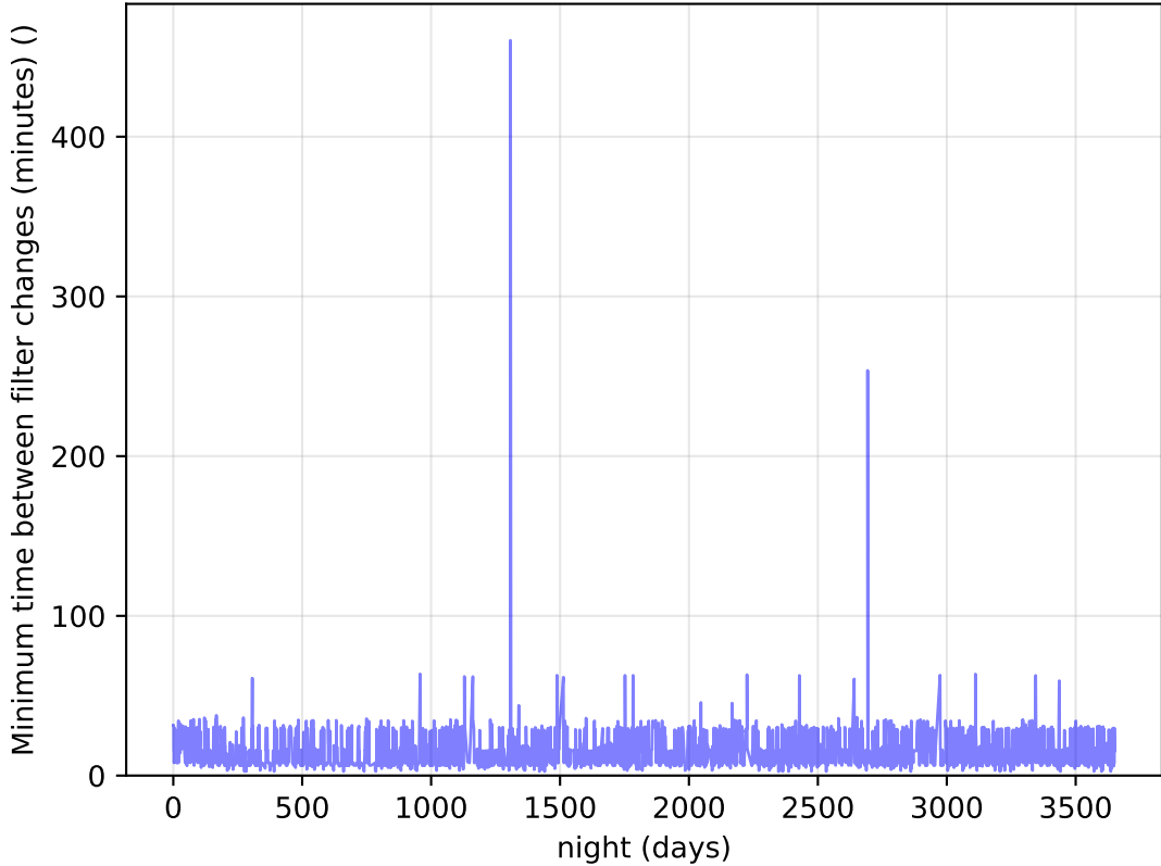
roll_uniform_eh_acc0.2_mjdp0_v3.4_10yrs Per Night: Minimum time between filter changes (minutes)
