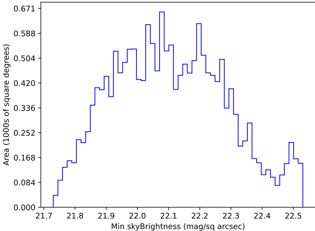
roll_uniform_eh_acc0.2_mjdp0_v3.4_10yrs WFD u band: Min skyBrightness
