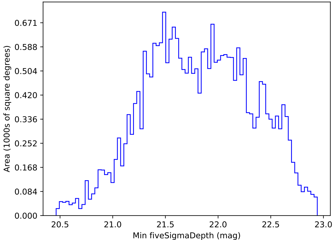
roll_uniform_eh_acc0.2_mjdp0_v3.4_10yrs All sky i band: Min fiveSigmaDepth
