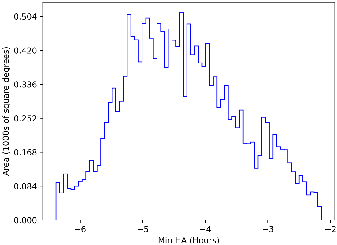
roll_uniform_eh_acc0.2_mjdp0_v3.4_10yrs WFD z band: Min HA
