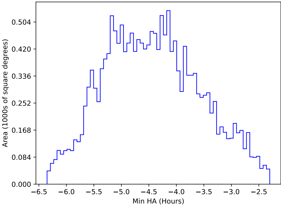
roll_uniform_eh_acc0.2_mjdp0_v3.4_10yrs WFD r band: Min HA
