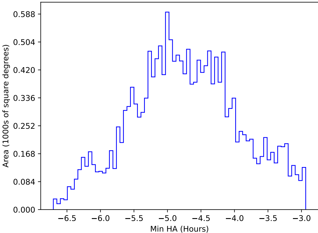
roll_uniform_eh_acc0.2_mjdp0_v3.4_10yrs WFD all bands: Min HA
