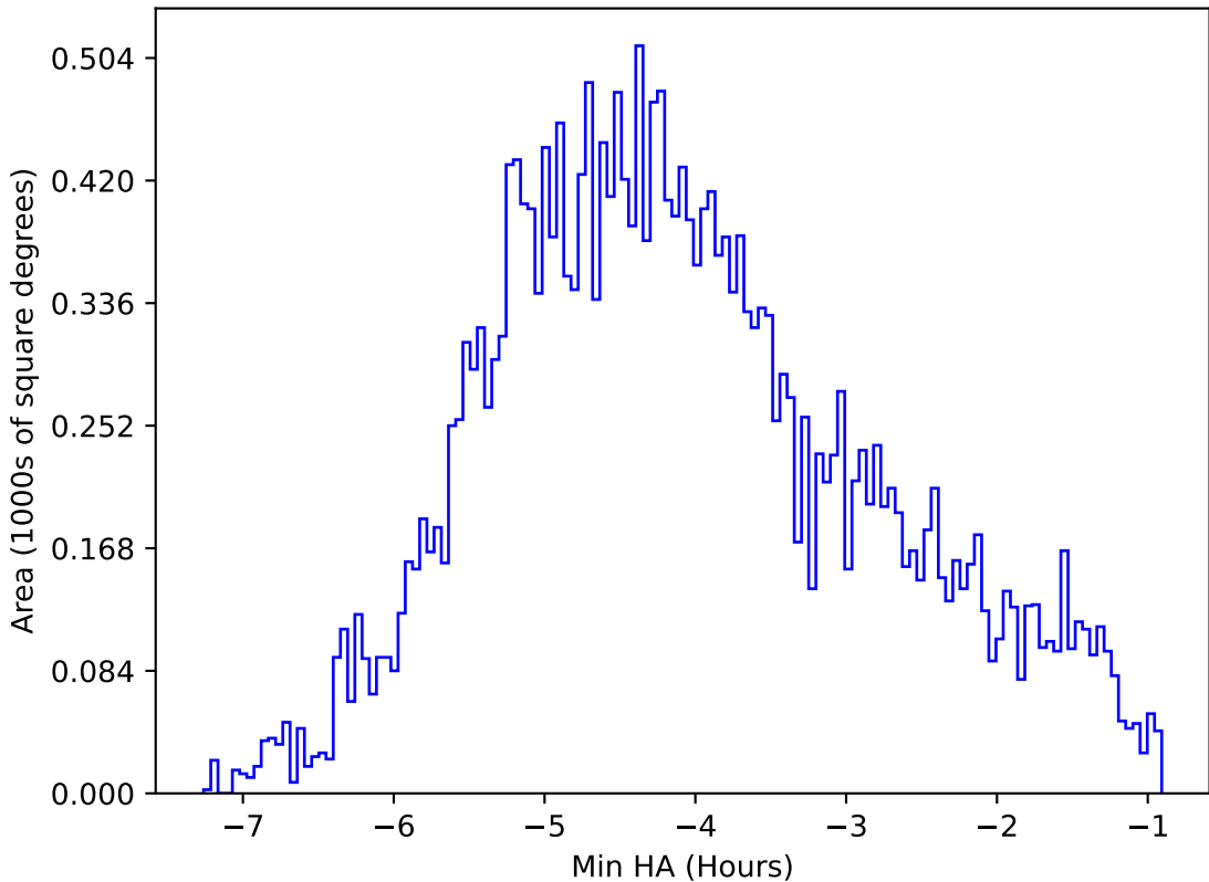
roll_uniform_eh_acc0.2_mjdp0_v3.4_10yrs All sky z band: Min HA
