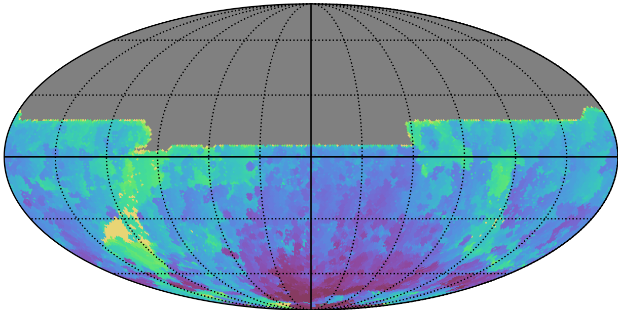
roll_uniform_eh_acc0.2_mjdp0_v3.4_10yrs All sky y band: Min HA
