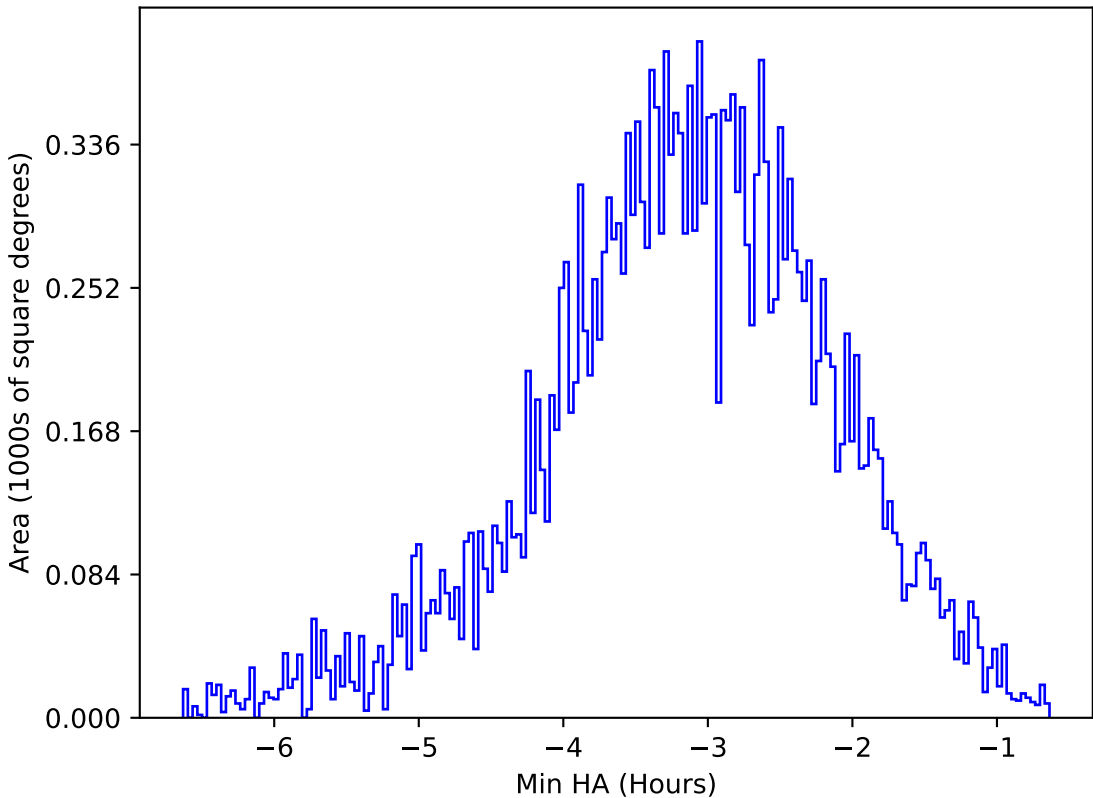
roll_uniform_eh_acc0.2_mjdp0_v3.4_10yrs All sky u band: Min HA
