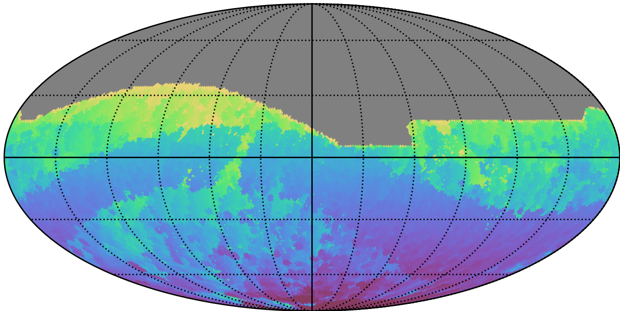
roll_uniform_eh_acc0.2_mjdp0_v3.4_10yrs All sky r band: Min HA
