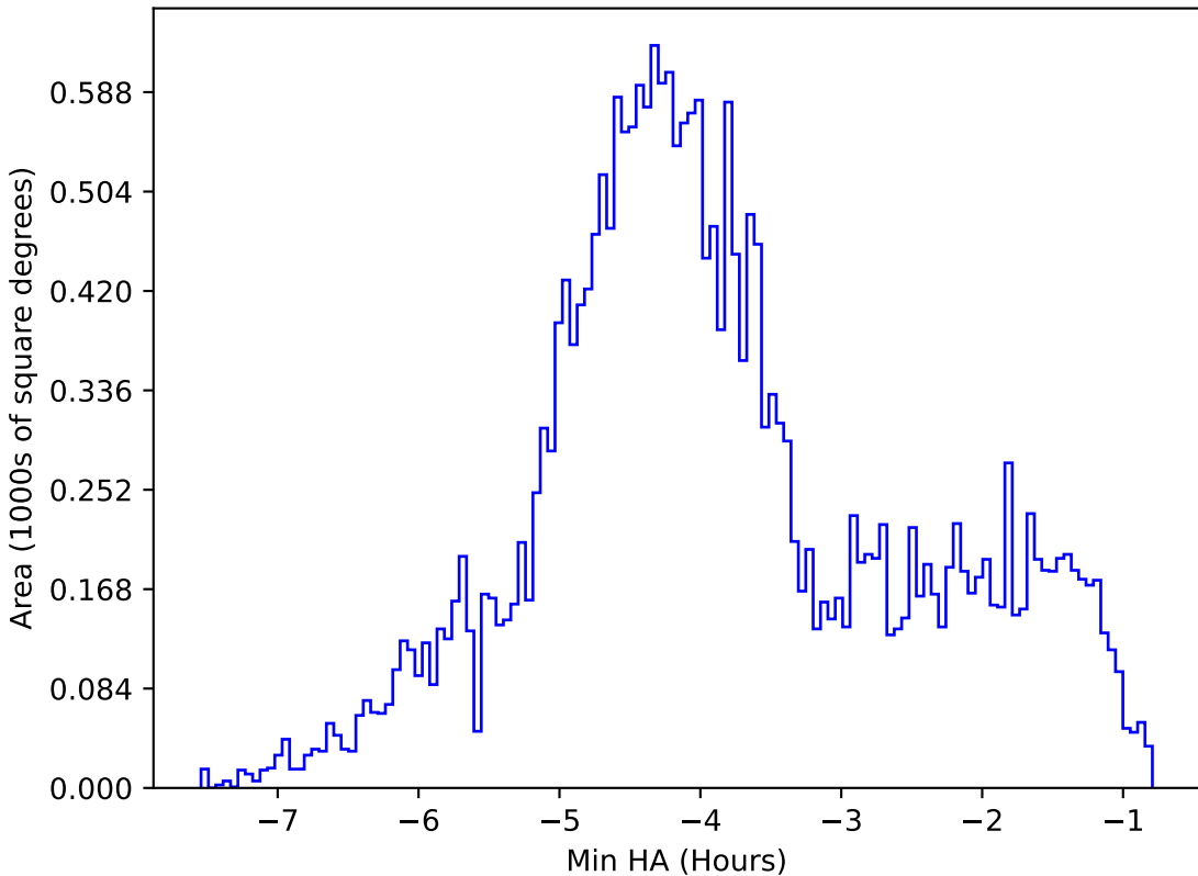
roll_uniform_eh_acc0.2_mjdp0_v3.4_10yrs All sky g band: Min HA
