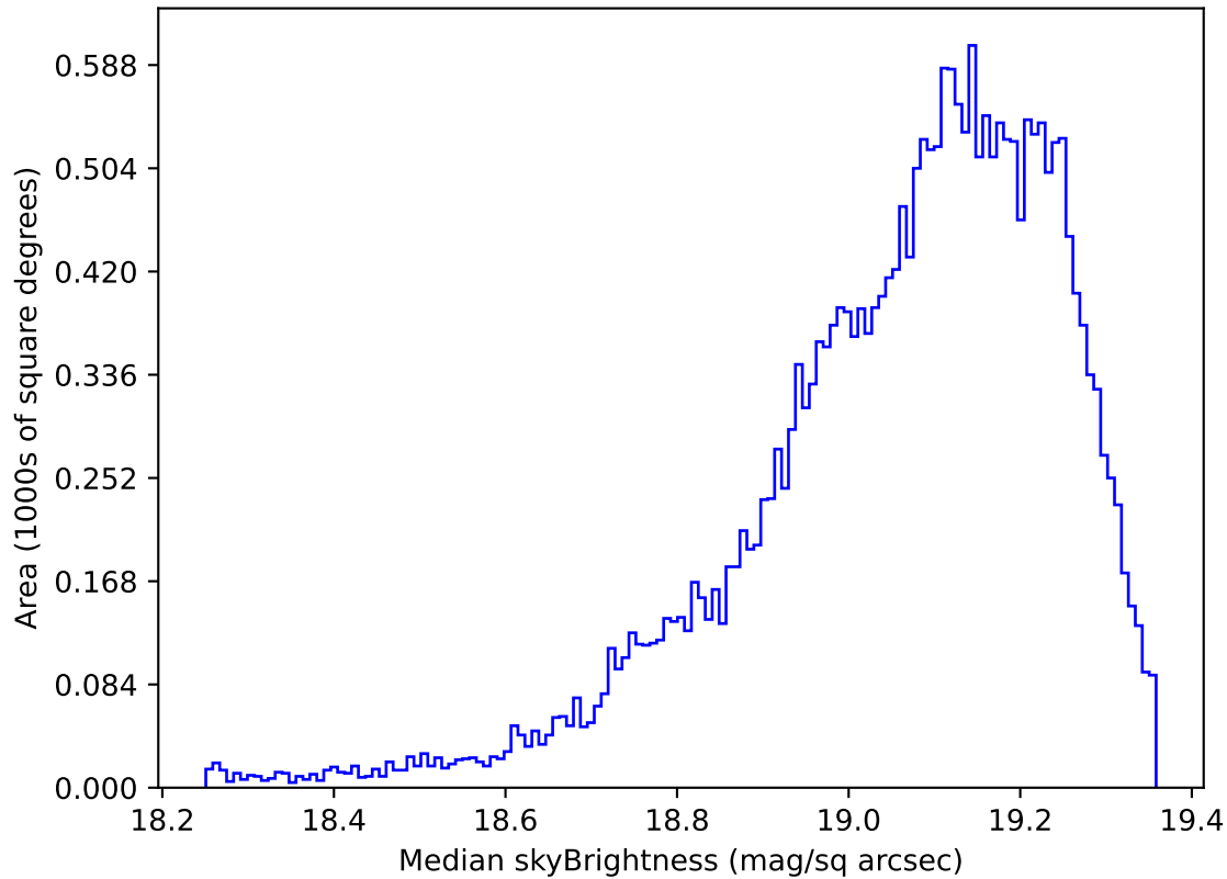
roll_uniform_eh_acc0.2_mjdp0_v3.4_10yrs Yr 1 z band: Median skyBrightness
