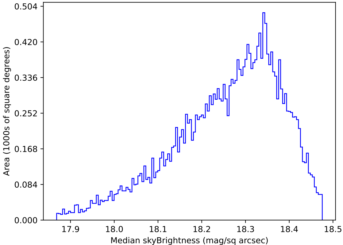
roll_uniform_eh_acc0.2_mjdp0_v3.4_10yrs Yr 1 y band: Median skyBrightness
