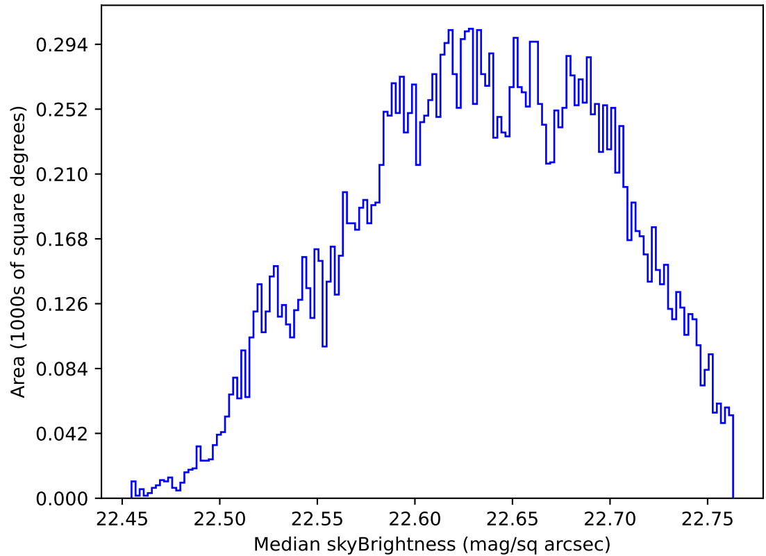
roll_uniform_eh_acc0.2_mjdp0_v3.4_10yrs Yr 1 u band: Median skyBrightness
