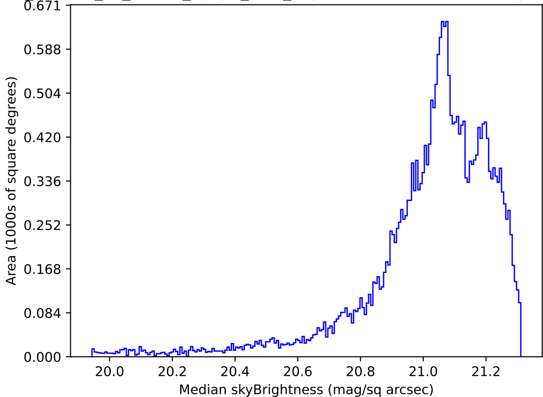
roll_uniform_eh_acc0.2_mjdp0_v3.4_10yrs Yr 1 r band: Median skyBrightness
