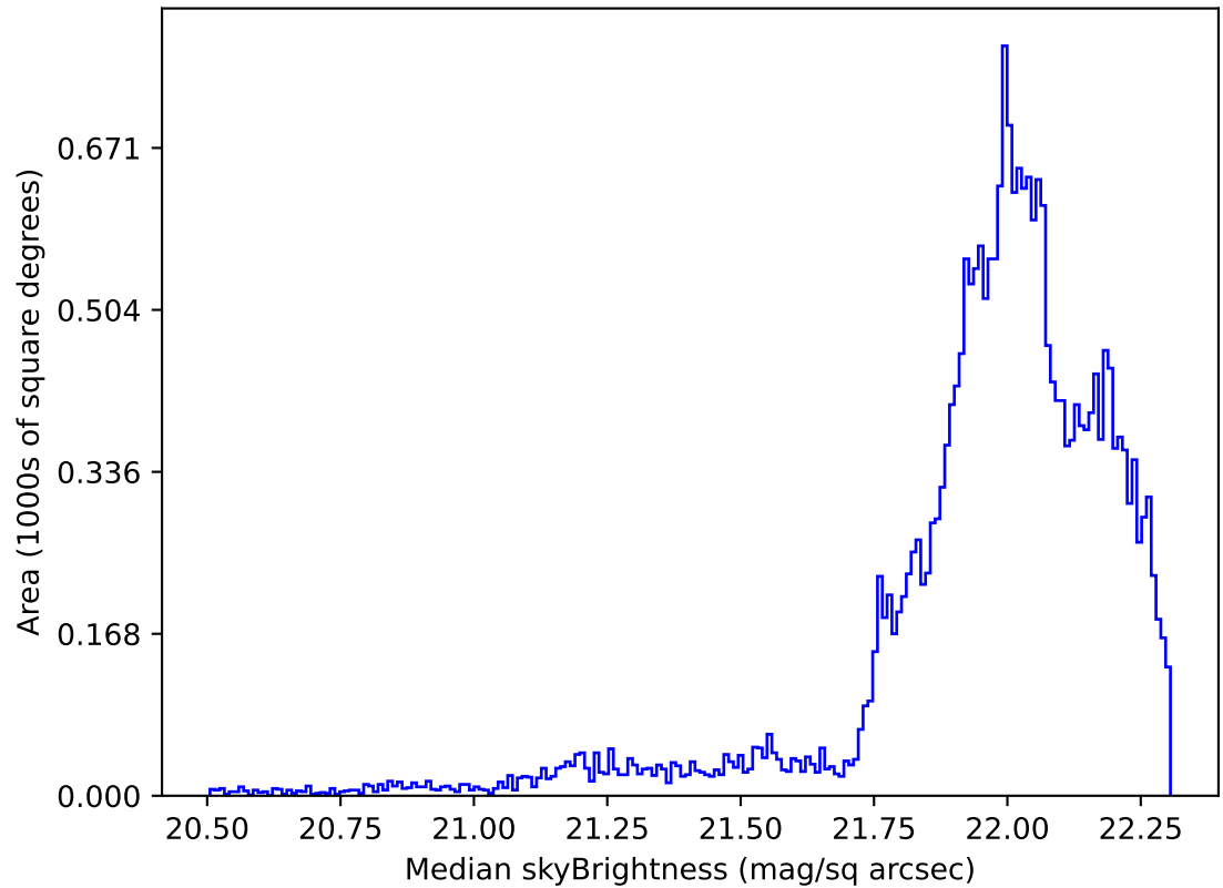
roll_uniform_eh_acc0.2_mjdp0_v3.4_10yrs Yr 1 g band: Median skyBrightness
