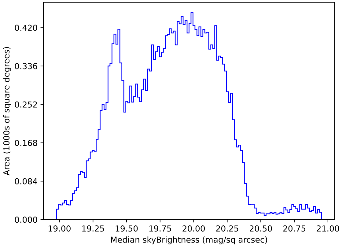
roll_uniform_eh_acc0.2_mjdp0_v3.4_10yrs Yr 1 all bands: Median skyBrightness
