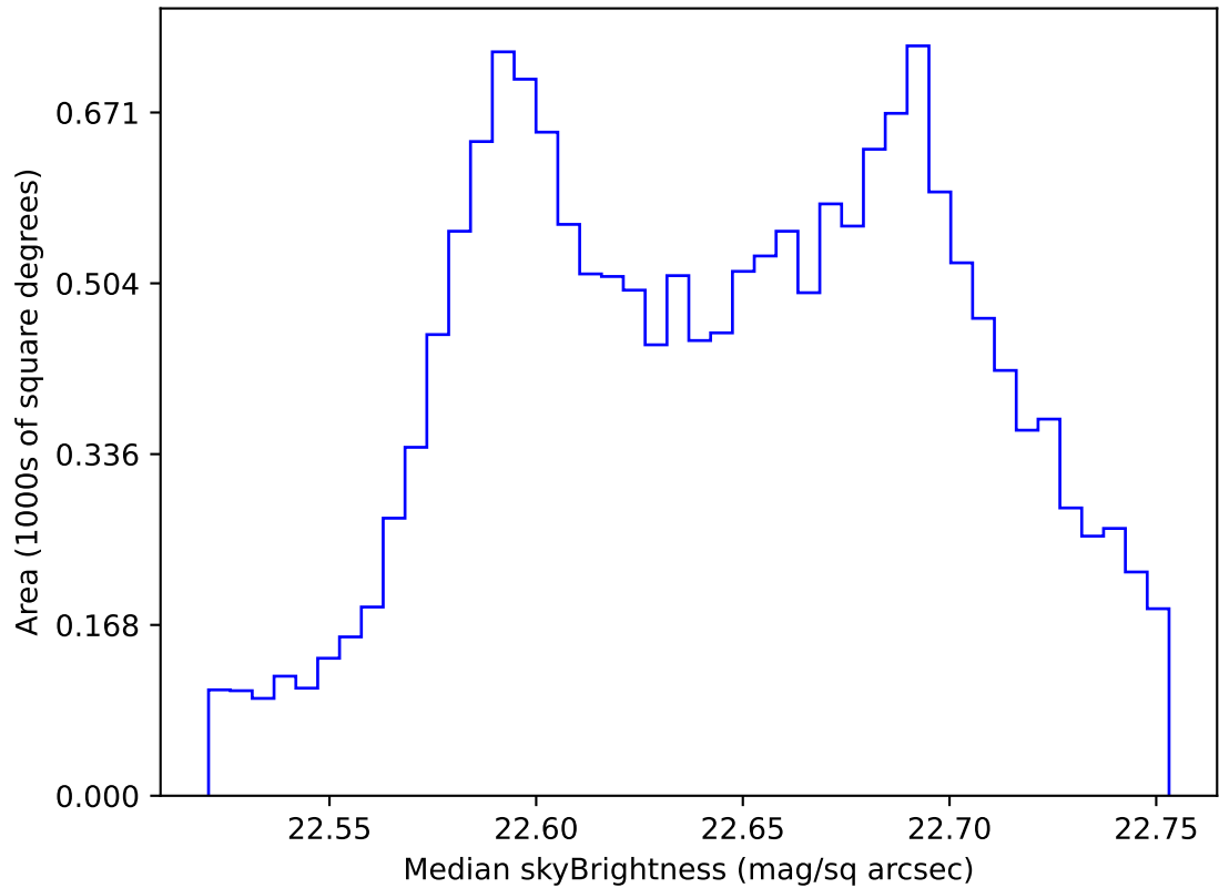
roll_uniform_eh_acc0.2_mjdp0_v3.4_10yrs WFD u band: Median skyBrightness
